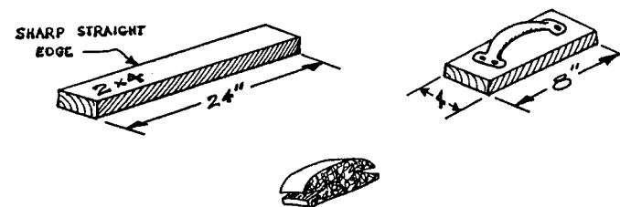
FIG. 5-6 SANDING BLOCKS
