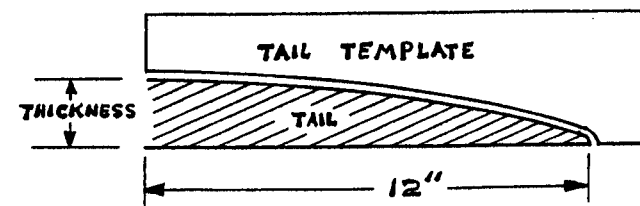
FIG. 3-11 TAIL CROSS-SECTION
