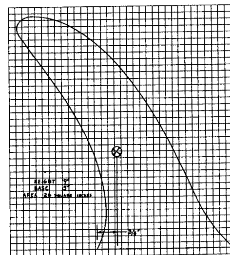
FIG. 4-17 FIN FOR TEARDROP SURFBOARD
