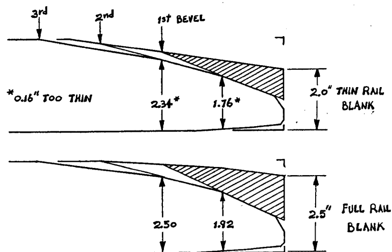
FIG. 6-1 EFFECT OF THIN RAIL ON BLANK
