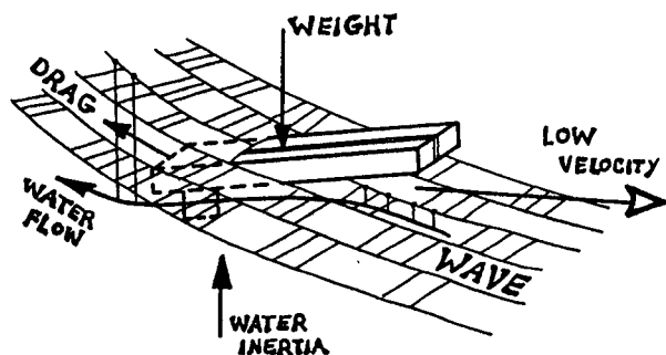
FIG. 2-17 PUSHING WATER
