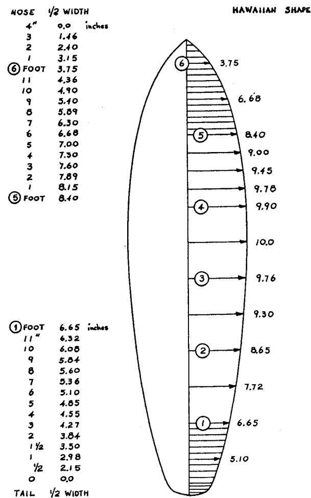
FIG. 4-21 6'4" HAWAIIAN SHAPE - RAIL OUTLINE
