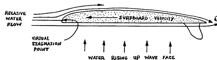
FIG. 2-30 RAIL FOIL
