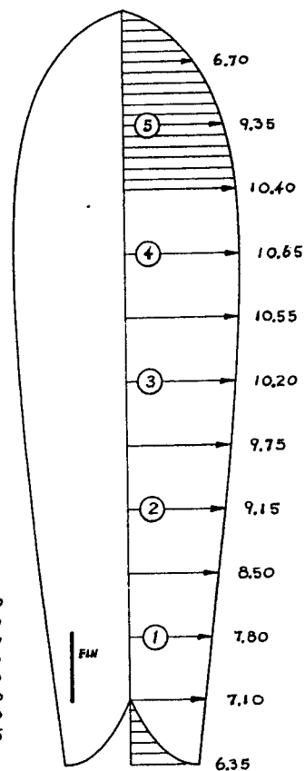
FIG. 4-18 5'11" FISH SURFBOARD - RAIL OUTLINE
