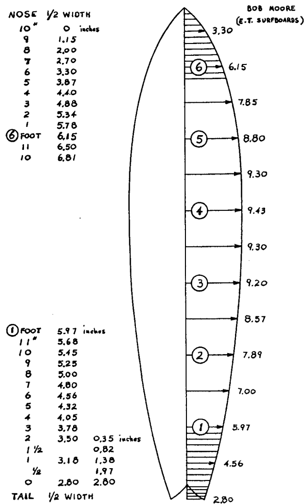
FIG. 4-11 6'10" SWALLOW TAIL - RAIL OUTLINE
