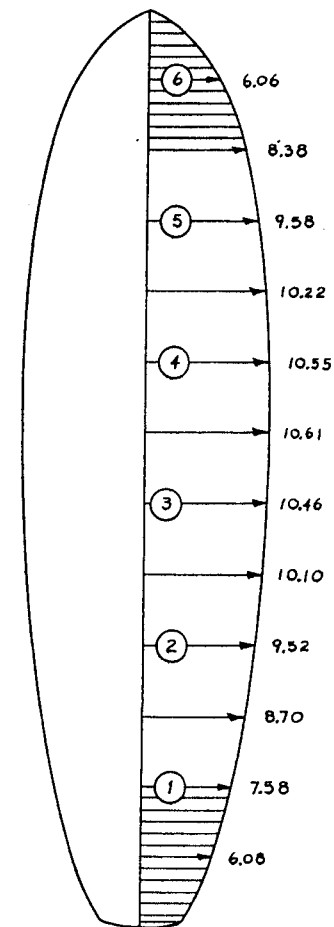
FIG. 4-7 6'6" ROUNDED SQUARE TAIL - RAIL OUTLINE
