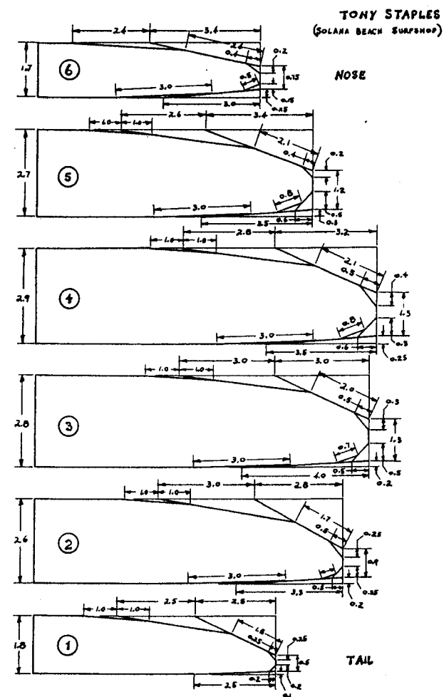
FIG. 4-5 6'8" EGG ROUND TAIL - RAIL CROSS-SECTIONS
